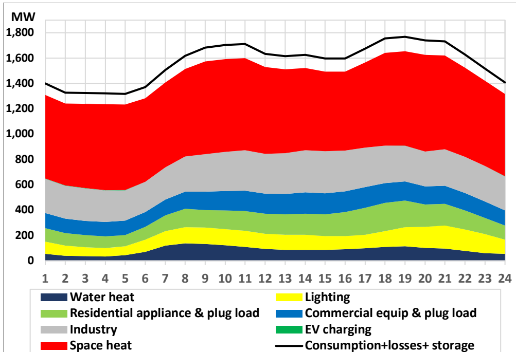
Figure 6. Average electricity consumption in winter, 2019 base year
